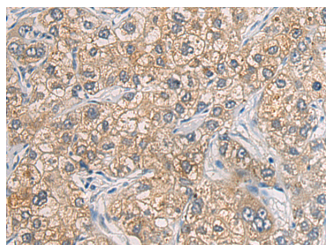
Immunohistochemistry of paraffin-embedded Human liver cancer tissue using GAB4 Polyclonal Antibody at dilution of 1:60(×200)
