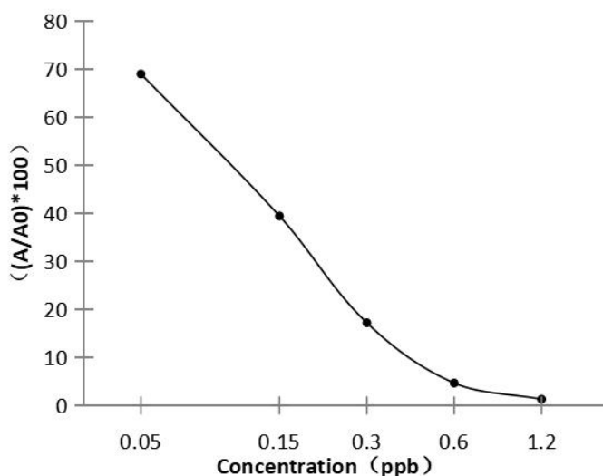
Ochratoxin A (E-TO-E021) Standard Curve
