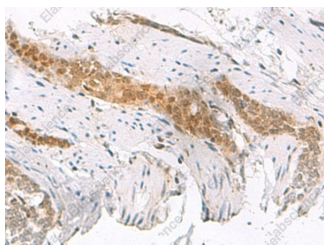
Immunohistochemistry of paraffin-embedded Human esophagus cancer tissue using SCAND1 Polyclonal Antibody at dilution of 1:50(×200)
