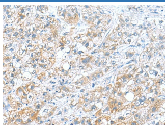
Immunohistochemistry of paraffin-embedded Human liver cancer tissue using DNAL1 Polyclonal Antibody at dilution of 1:70(×200)
