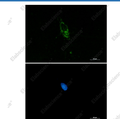
Immunofluorescent analysis of HCT116 cells using Pumilio 1 Monoclonal Antibody (green), and DAPI (blue).
