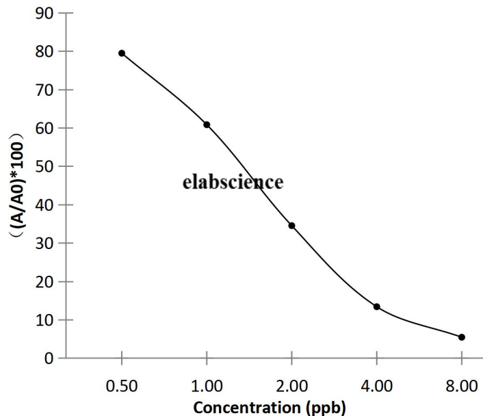
Spectinomycin (E-FS-E081) Standard Curve
