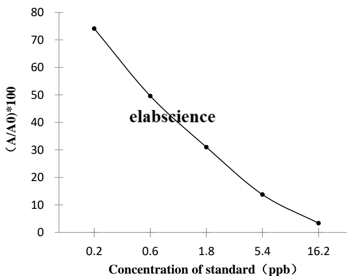
Pentachlorophenol Sodium (E-FS-E093) Standard Curve
