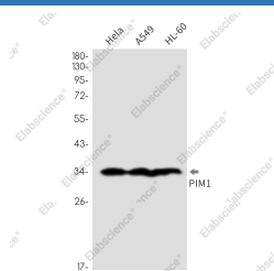
Western Blot analysis of HeLa,A549,HL-60 cells using PIM1 Monoclonal Antibody.
