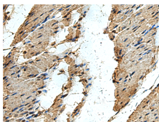
Immunohistochemistry of paraffin-embedded Human thyroid cancer tissue using ERLIN1 Polyclonal Antibody at dilution of 1:50(×200)
