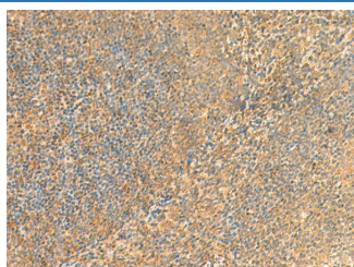
Immunohistochemistry of paraffin-embedded Human tonsil tissue using UBD Polyclonal Antibody at dilution of 1:50( \times 200 )
