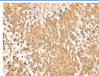
Immunohistochemistry of paraffin-embedded Human lung cancer tissue using UBD Polyclonal Antibody at dilution of 1:50( \times 200 )
