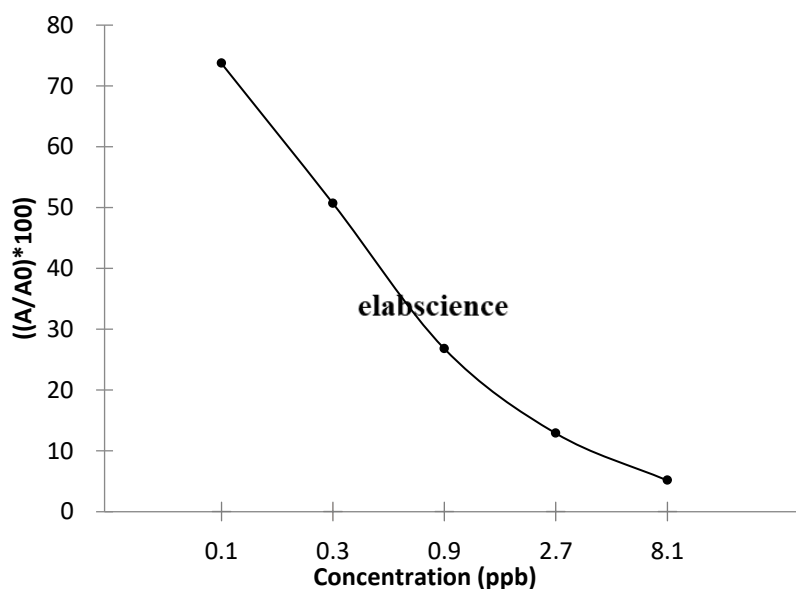
Trimethoprim (E-FS-E153) Standard Curve
