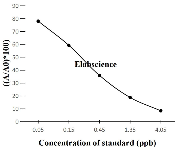
Total Aflatoxin (E-TO-E026) Standard Curve
